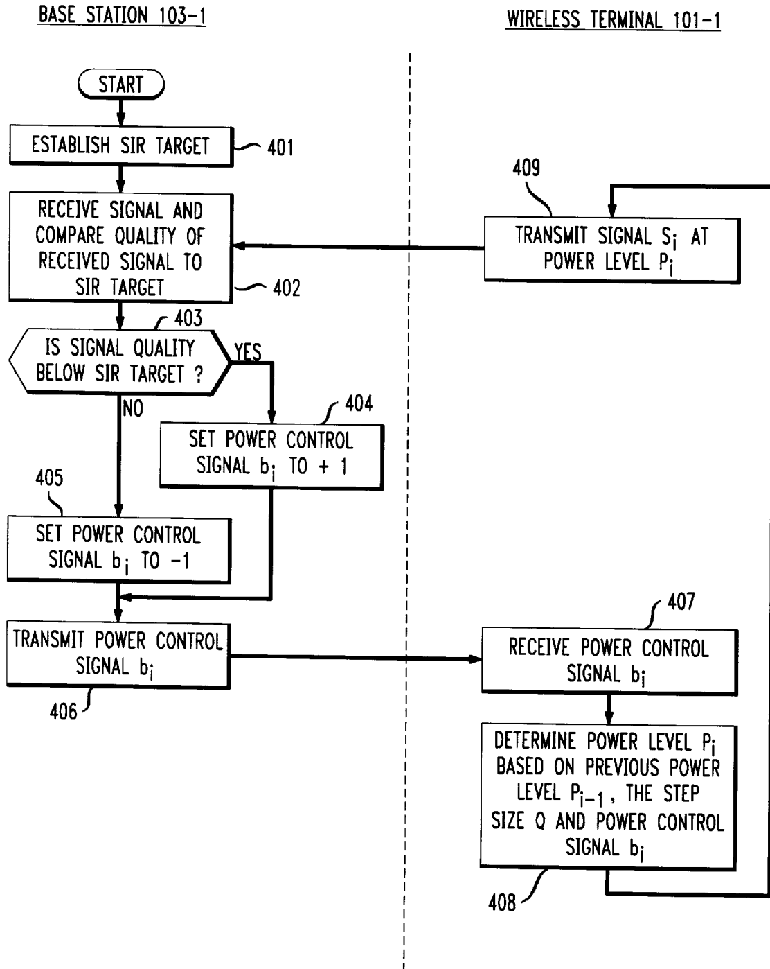
FIG. 4 PRIOR ART
